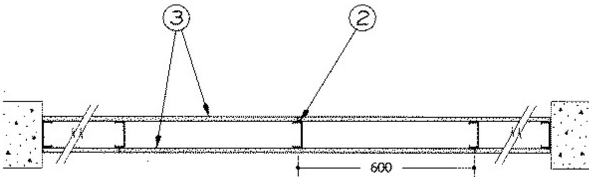
HORIZONTAL SECTION
