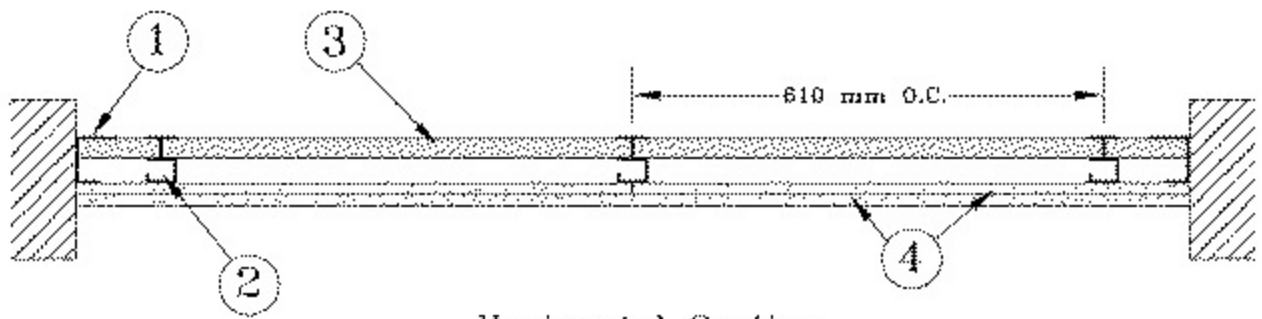
Horizontal Section
