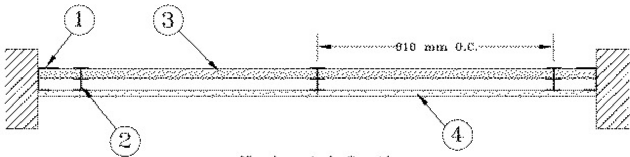
Horizontal Section
